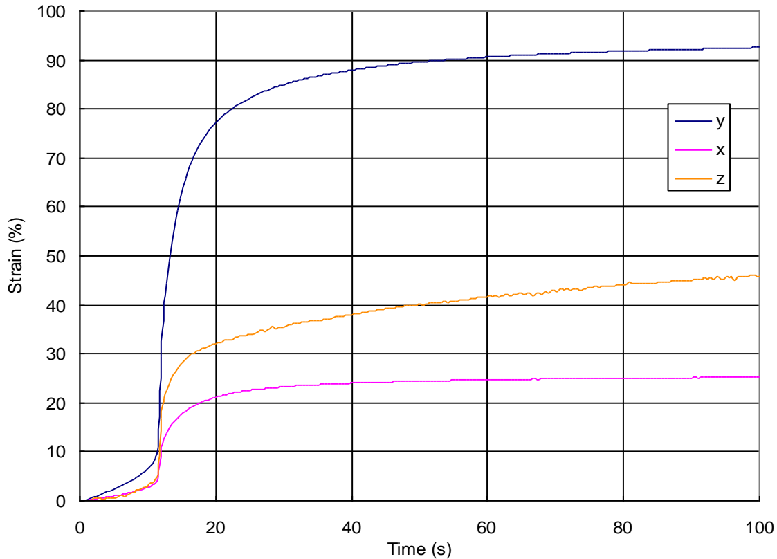
Fig. 3: A rapid increase in strain is noted at yield
