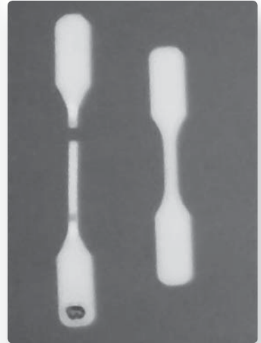
Test specimens of a plastic before and after a test. "Necking," or the narrowing and stretching of the high stress area, is visible on the left.
